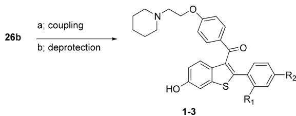
Scheme 7. (a) Compound 13 , 20 or 25 , Pd(PPh 3 ) 4 , DMF, 100 °C, 12 h, (b) n -Bu 4 NF· x H 2 O, THF, rt, 1 min, 47% (compound 1 ; including MOM deprotection, concd HCl in isopropanol, 60 °C, 30 min), 68% (compound 2 ) or 80% (compound 3 ).
