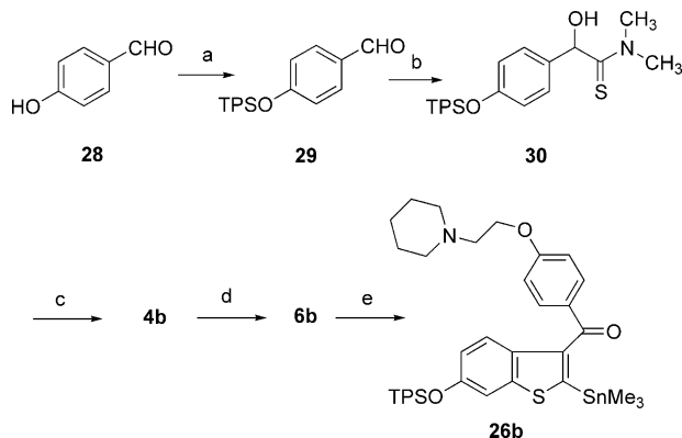
Scheme 6. (a) TPSCl, imidazole, DMF, rt, 3 h, 99%; (b) N,N -dimethylthioformamide, LDA, THF/hexane (5:1), –100 to –78 °C, 1 h, 57%; (c) methanesulfonic acid, CH 2 Cl 2 , –10 °C, 10 min, 49%; (d) compound 5 , chlorobenzene, 100 °C, 9 h, 68%; (e) LiMe 3 Sn, THF, –78 °C to rt, 5 h, 71%.
