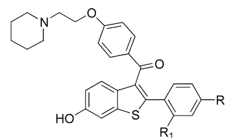
1: R 1 = CH 2 CH 2 CH 2 F, R 2 = OH 2: R 1 = CH 2 CH 2 CH 2 F, R 2 = H 3: R 1 = CH 2 CH 2 F, R 2 = H
