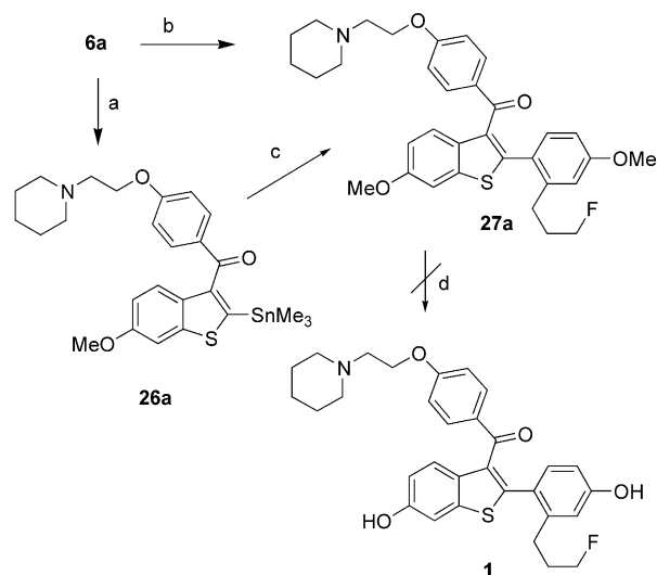
Scheme 5. (a) LiMe 3 Sn, THF, –78 °C to rt, 5 h, 99%; (b) 2-(3-fluoropropyl)-4-methoxyphenylmagnesium bromide, THF, –78 °C to rt, 2 h, 60%; (c) compound 13 , Pd(PPh 3 ) 4 , DMF, 120 °C, 9 h, 57%; (d) BBr 3 , CH 2 Cl 2 , rt, 1 h or AlCl 3 , CH 3 CH 2 SH, CH 2 Cl 2 , rt, 1 h or SiCl 4 , NaI, CH 2 Cl 2 , rt, 1 h or CH 3 SiH, CHCl 3 , rt, 1 h.
