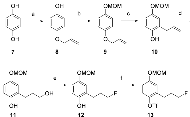
Scheme 2. (a) Allyl bromide, K 2 CO 3 , CH 3 CN, reflux, 12 h, 92%; (b) MOMCl, NaH, THF, 0 °C to reflux, 1 h, 92%; (c) N,N -dimethylaniline, reflux, 2 h, 80%; (d) borane–THF complex, H 2 O 2 , 4N NaOH, THF, 0 °C, 1 h, 78%; (e) DAST, CH 2 Cl 2 , –78 °C to rt, 30 min, 15%; (f) Tf 2 O, 2,6-lutidine, CH 2 Cl 2 , 0 °C to rt, N 2 , 30 min, 92%.
