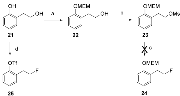
Scheme 4. (a) MEMCl, NaH, THF, 0 °C to reflux, 1 h, 70%; (b) MsCl, Et 3 N, CH 2 Cl 2 , 0 °C, 20 min, 82%; (c) n -Bu 4 NF·xH 2 O, CH 3 CN, 110 °C, 30 min, obtained vinyl compound; (d) (i) DAST, CH 2 Cl 2 , –78 °C to rt, 30 min; (ii) Tf 2 O, 2,6-lutidine, CH 2 Cl 2 , 0 °C to rt, N 2 , 30 min, 26%.
